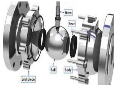
METAL SEATED VALVE CONNECTION TYPE: ANSI 150-600#RF FLANGED SIZES: 1/2" - 6" MATERIAL: CARBON / STAINLESS STEEL
